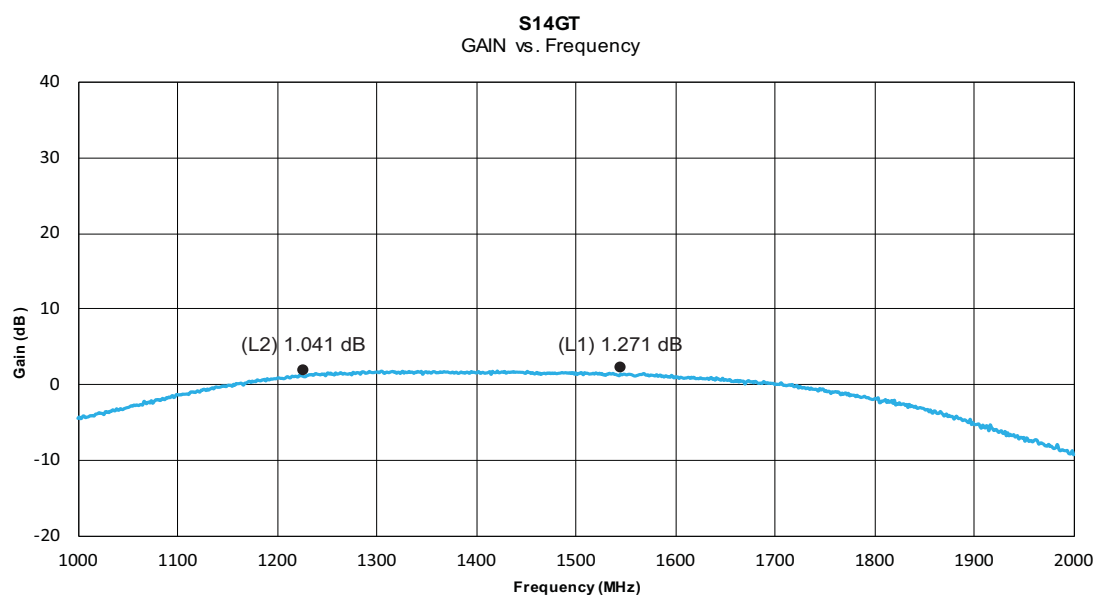
Figure 2-4. Frequency Response (0dB)
