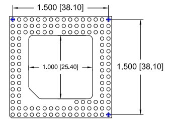
Fig.35 127 Pins
