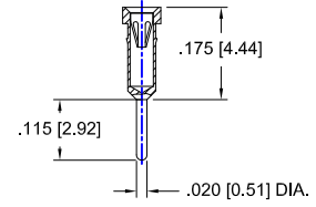
- 01 Terminal Shown
